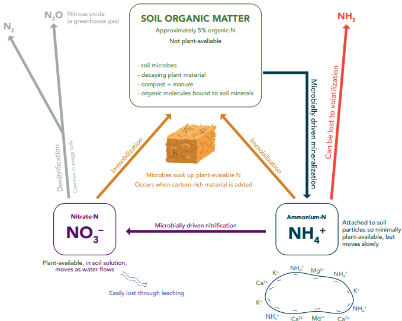
Figure 3. Soil nitrogen pools and pathways.
