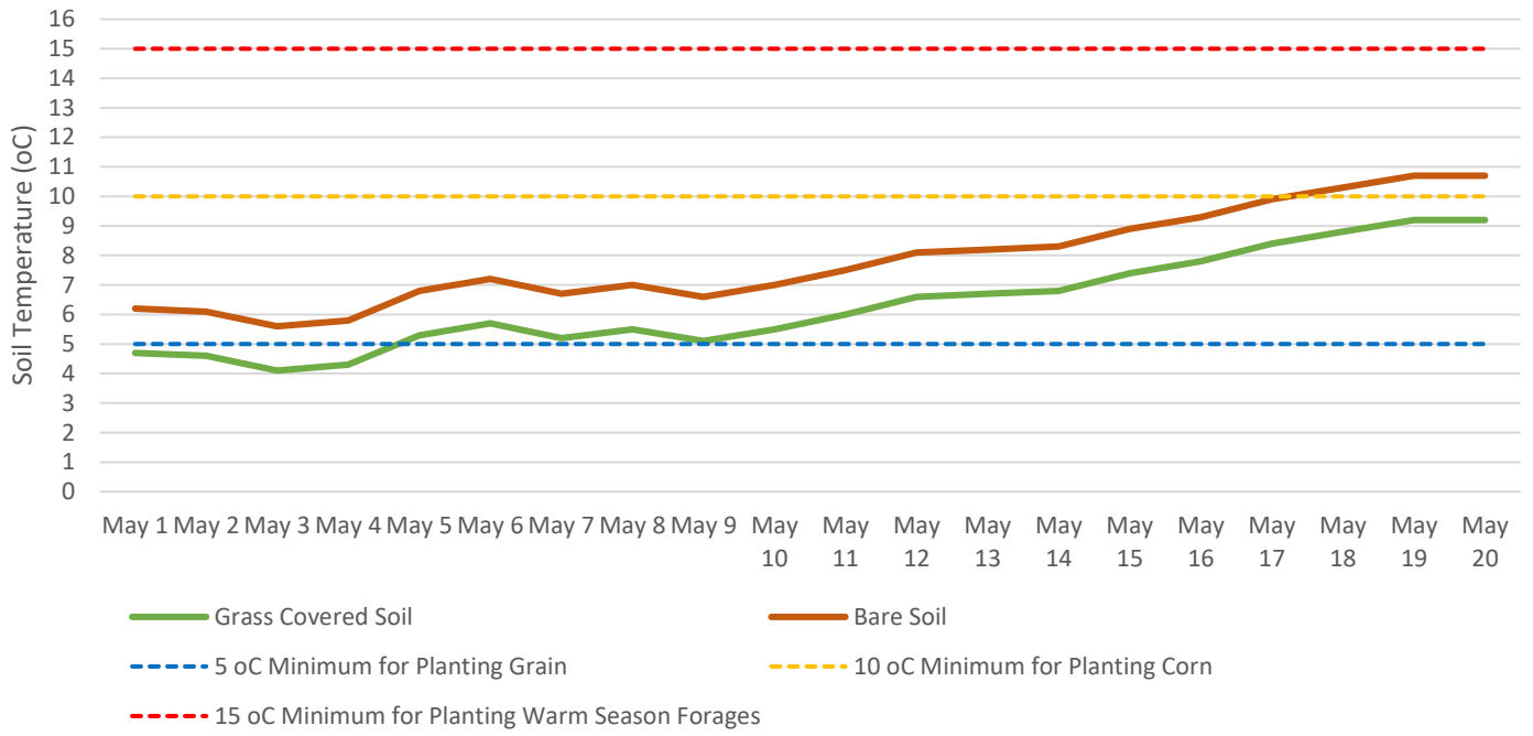
Perth Soil Temperature at 6" Depth
